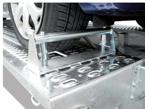
Radstopper
